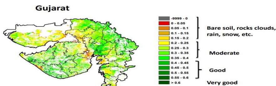
NOAA/VIIRS/BLENDED NDVI Composite ending on Week no 39 (24.09.2022 to 30.09.2022) over Agricultural region
