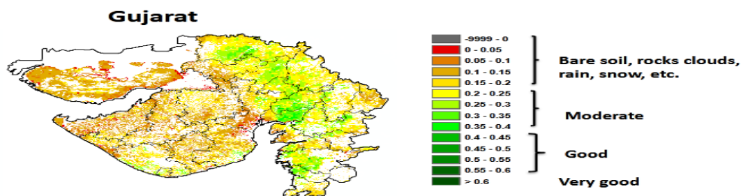
NOAA/VIIRS/BLENDED NDVI Composite ending on Week no 15 (09.04.2023 to 15.04.2023) over Agricultural region
