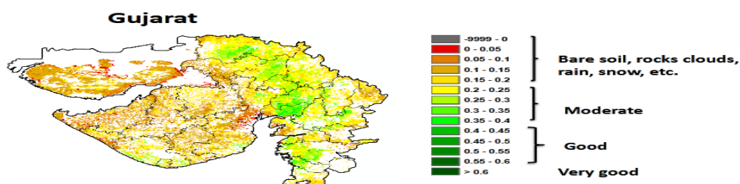
NOAA/VIIRS/BLENDED NDVI Composite ending on Week no 15 (09.04.2023 to 15.04.2023) over Agricultural region
