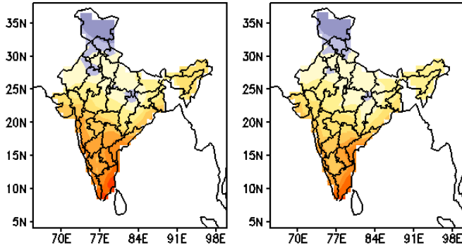
MME Bias corrected forecast Tmin (Deg)
