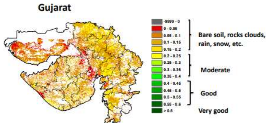
NOAA/VIIRS/BLENDED NDVI Composite ending on Week no 32 (06.08.2021 to 12.08.2021) over Agricultural region
